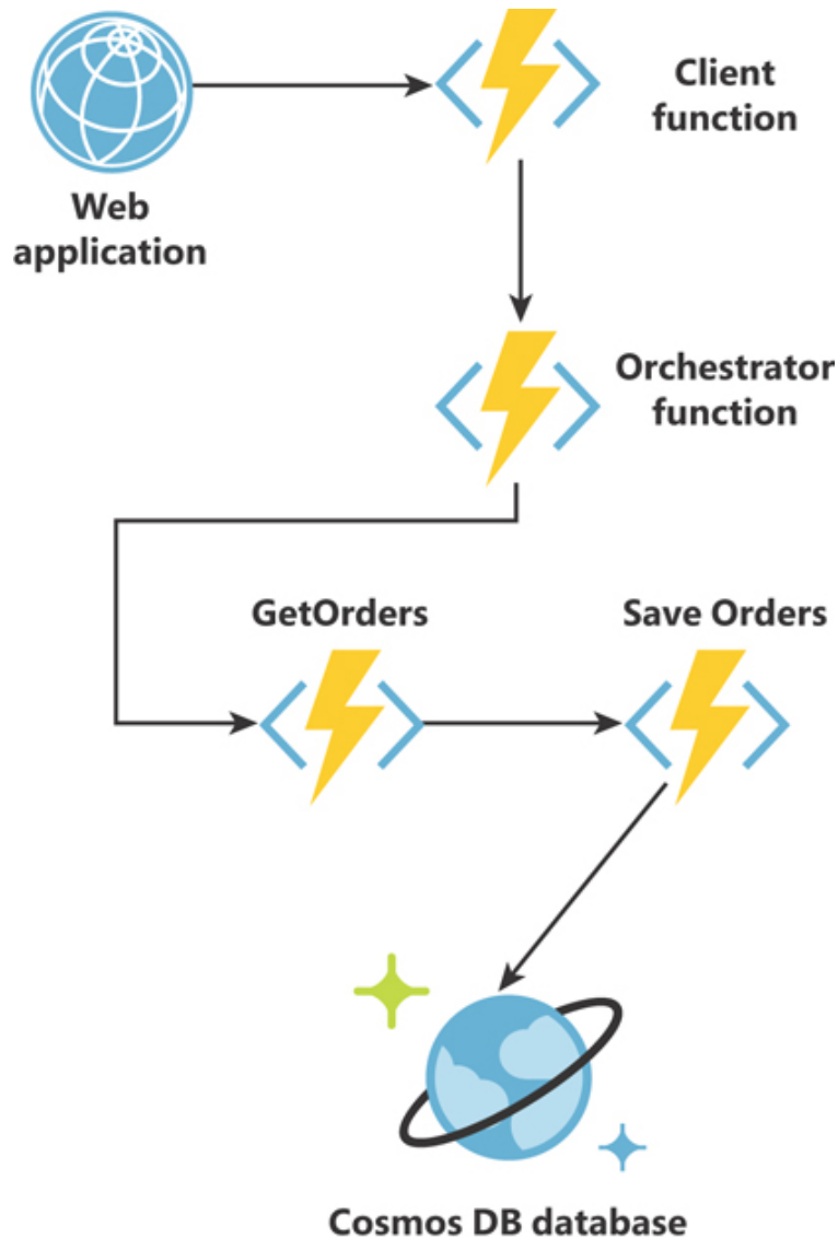
Figure 1-13 Durable function workflow
